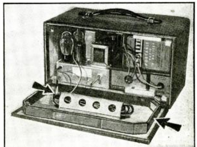
Rear view of the model BP5 portable showing (arrow at left) the A.C.-D.C. line cord; and (arrow at right) the built-in loop antenna. The self-contained batteries also are shown.
