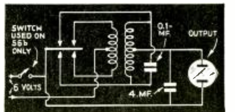
THE POWER PACK FOR DRY SHAVERS, shown as The Radiart Corp.'s item No. 1683 in Oct., 1938, Radio-Craft , is diagrammed above. Transformer has split primary, each half rated at 2.8 A. at 6 V. or 0.5-A. at 32 V. Secondary, also split, is rated at 100 ma. at 110 W. (each half).
