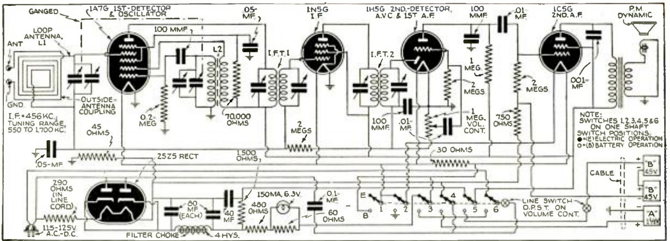
Fig. 1. Complete schematic diagram of the first receiver to operate optionally from both 110 V. A.C. or D.C. and self-contained batteries—using the new 1.4-V. low-drain tubes.
