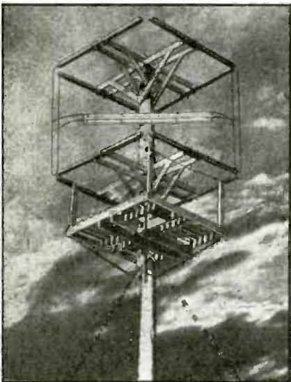
CUBIC TELEVISION ANTENNA FOR W2XB
